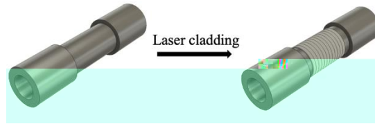
Fig.1 Work piece before and after laser cladding process.
