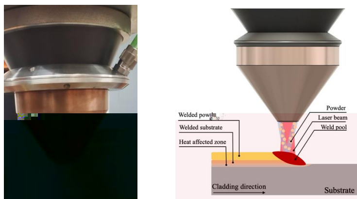
Fig.3 (a) Powder feeding (b) Schematics of coaxial powder feeding laser cladding.
