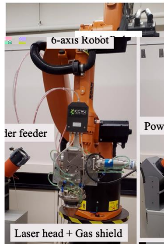
Fig.2 experiment Equipment.
