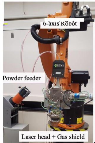
Fig.2 experiment Equipment.
