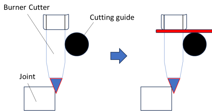
Fig. Idea of Cutting Guide.
