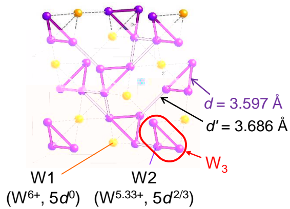
\text{CsW}_2\text{O}_6 -58 °C P2_13 (Phase II)
